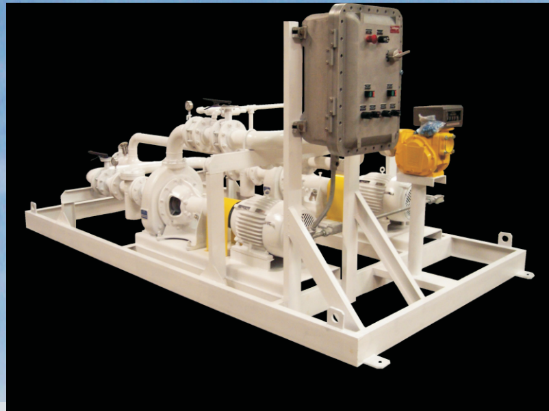
Duplex JP-8 Fuel Transfer Skid US Army-Camp Balad, Iraq
